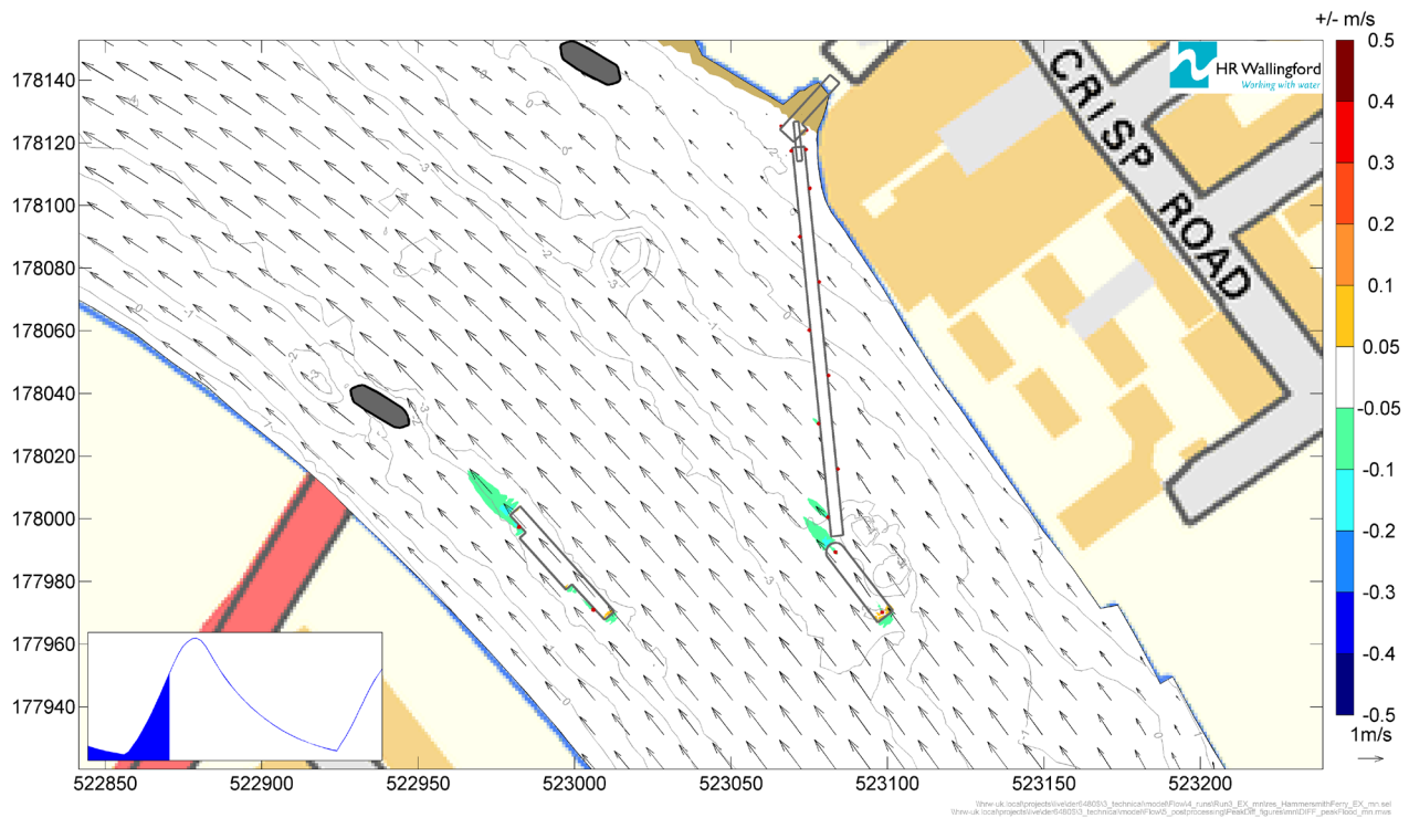
Figure 3.6: Difference in peak flood depth averaged currents associated with the proposed changes
