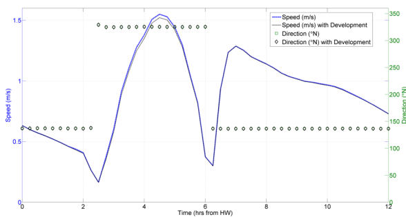
Figure 3.13: Position 1: Temporal variation in current speed and direction for baseline and proposed cases
