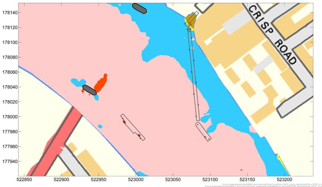
Figure 3.21: Baseline conditions: bed material summary based on peak bed shear stress – MN scenario
