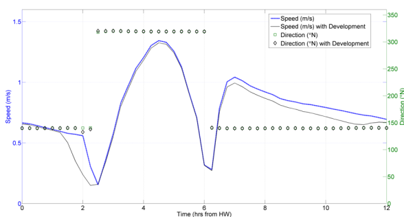
Figure 3.15: Position 3: Temporal variation in current speed and direction for baseline and proposed cases
